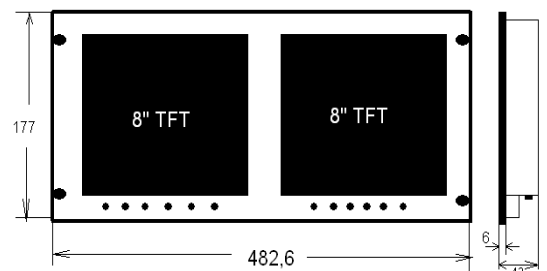
Dual Rack Panel PC
