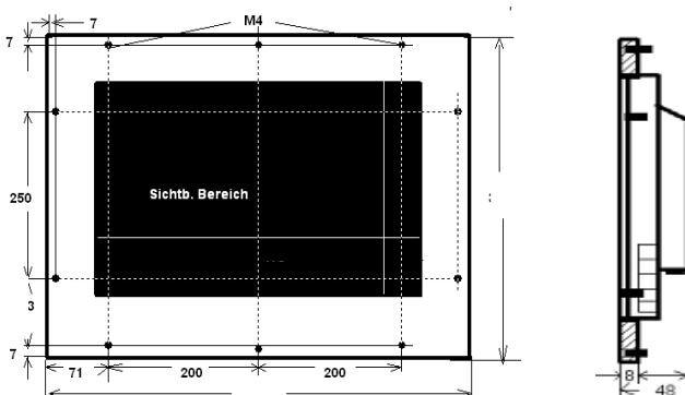
24" Panel-Mounting
