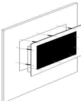
Panel Mounting
