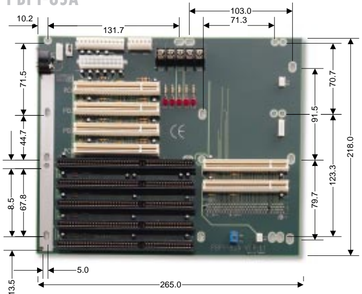
PBPI-8SA
