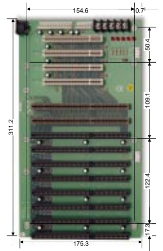
PBI-14SB
