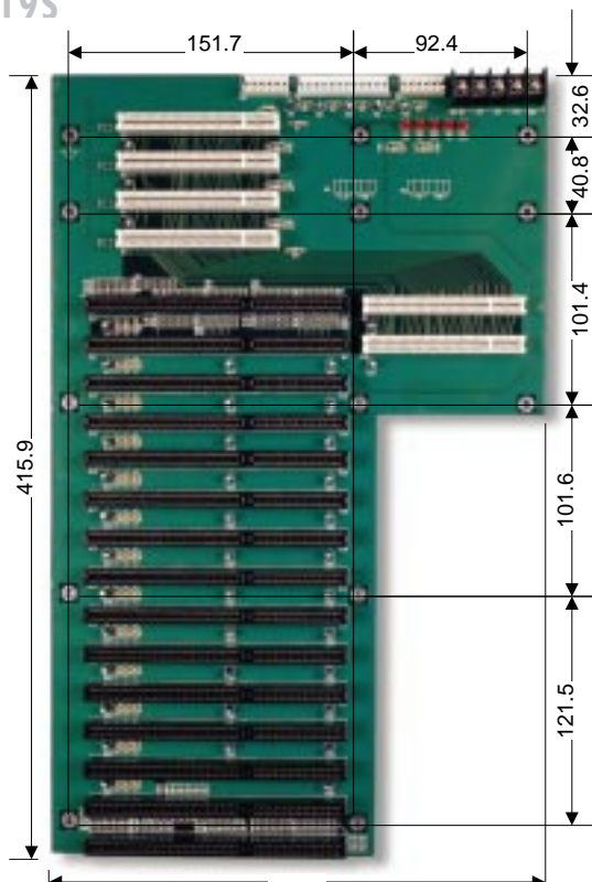
PBPI-19S
