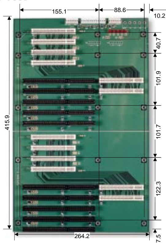
PBPI-18SD
