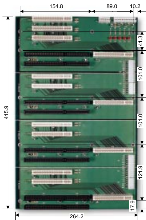
PBPI-17SQ
