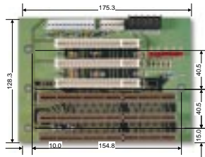
PBI-5S
