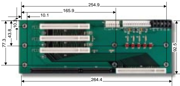
PBPI-4S
