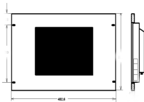
Rack (=19“) Mounting
