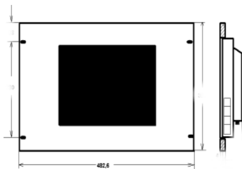
Rack (=19“) Mounting
