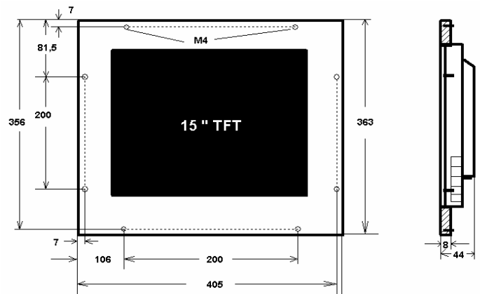
15,1" Panel-Mounting
