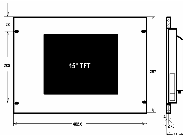
15,1" Rackmounting (19")
